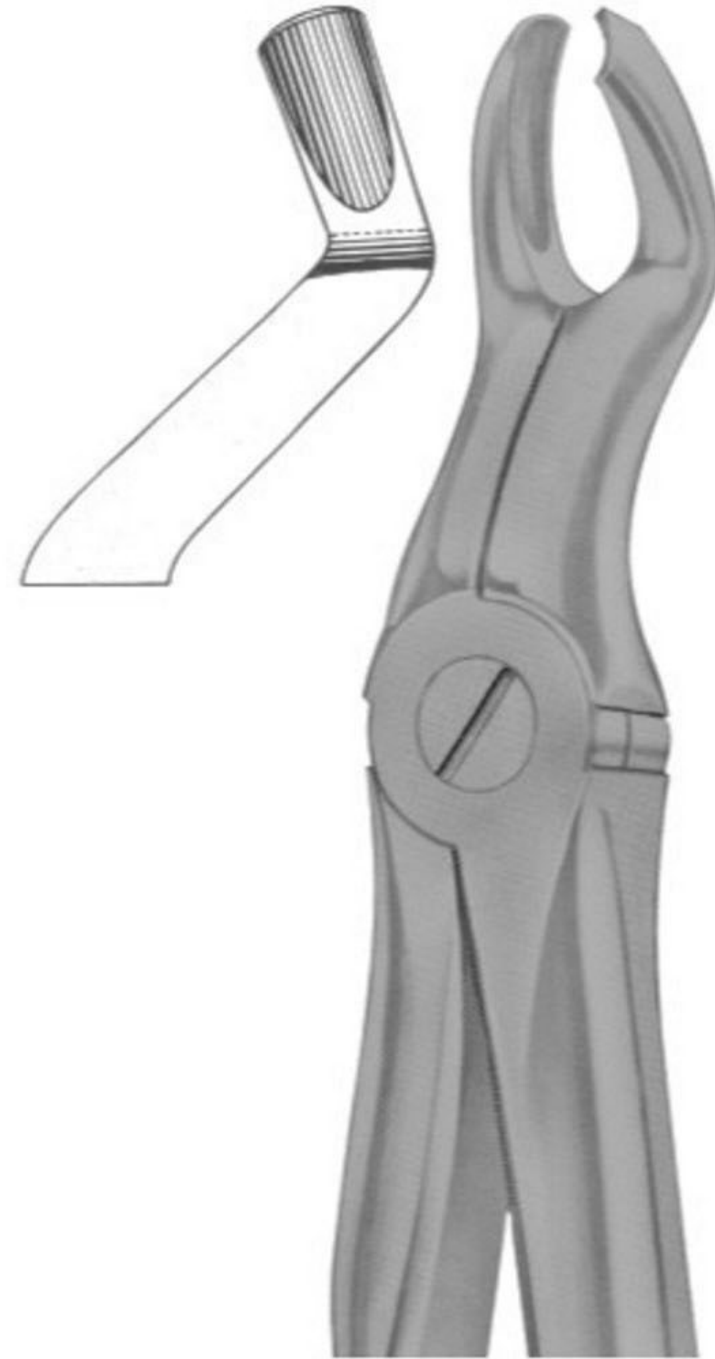
1188 Fig. 67 ½ L upper third molars left
