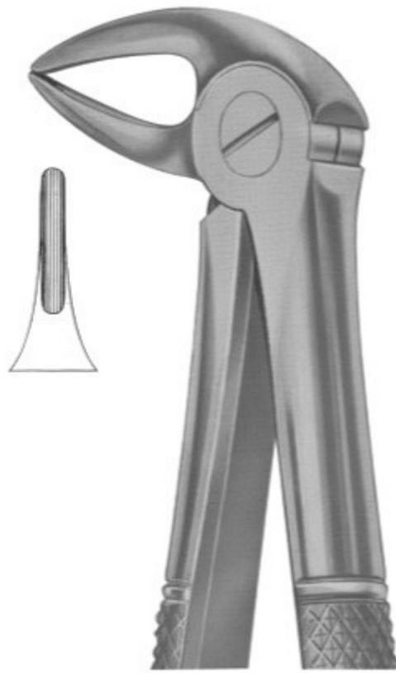
1030 Fig. 33A lower roots
