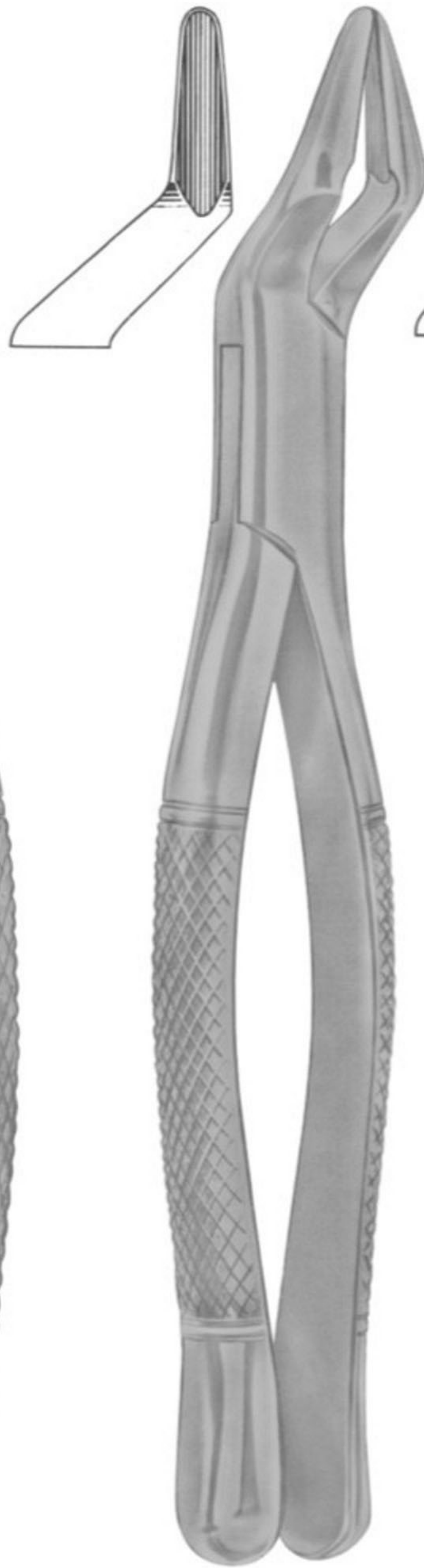
1247 PARMLY Fig. 32 upper premolars and molars
