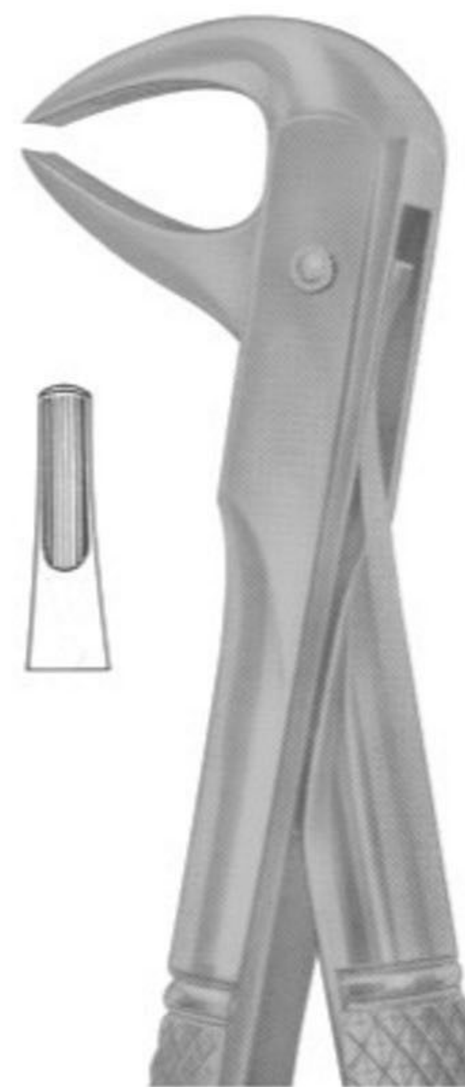
1071 Fig. 74D lower roots
