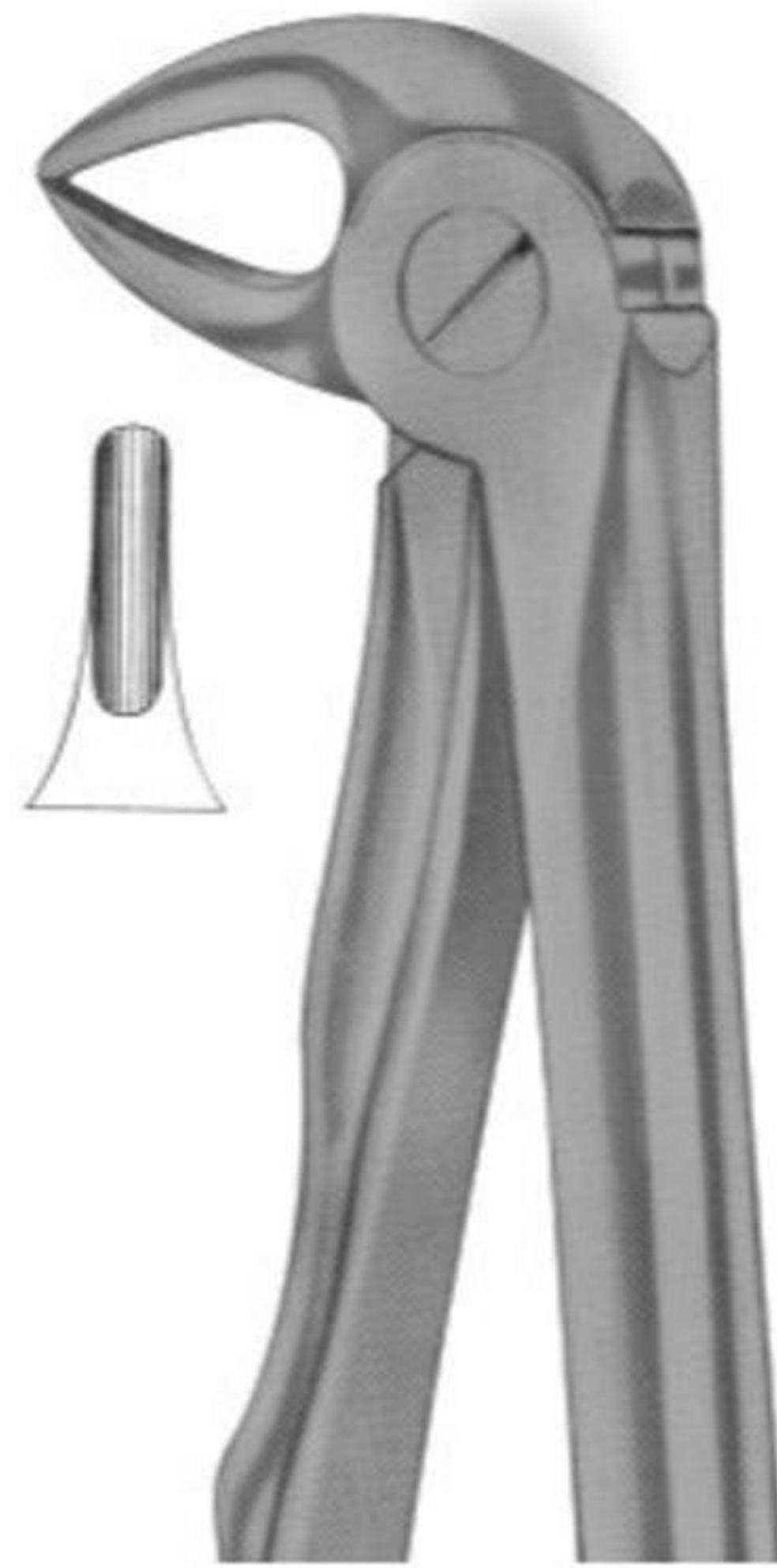
1167 Fig. 33S lower roots for children
